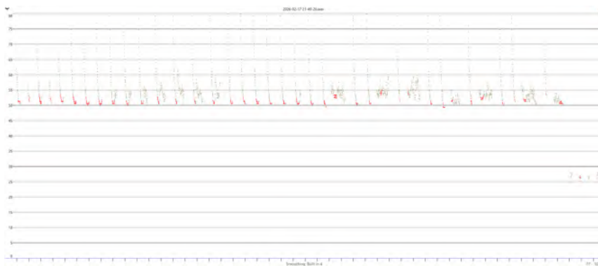
Figure 4-9: Vespadelus vulturnus definite call
