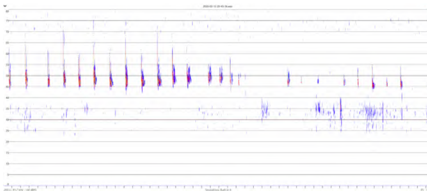
Figure 4-5: Miniopterus orianae oceanensis probable call – F5 uncompressed spectrogram view showing characteristic single-phase feeding buzz
