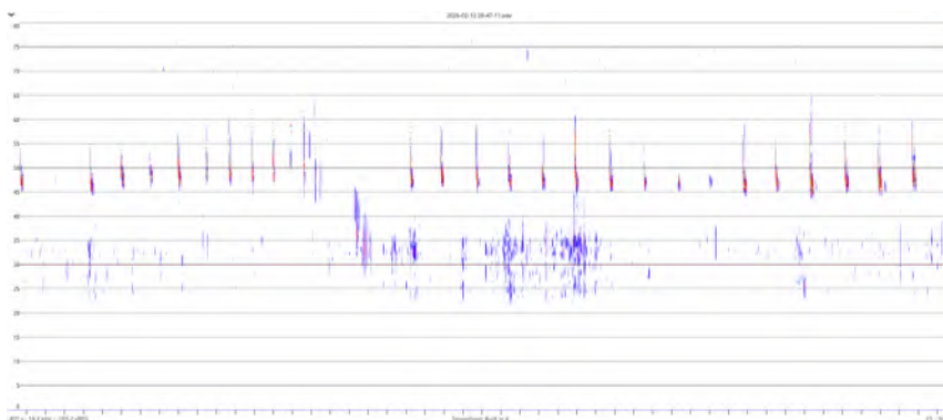
Figure 4-8: Vespadelus regulus definite call – F5 uncompressed spectrogram view showing characteristic two-phase feeding buzz
