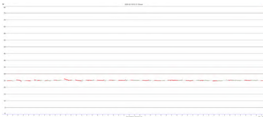
Figure 4-6: Ozimops planiceps possible call – outside of species distribution
