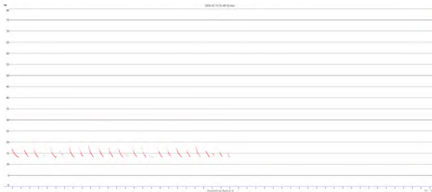
Figure 4-1: Austronomus australis definite call
